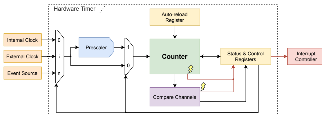
Figure 2.1: Core components and functional overview of a basic hardware timer. Interrupt event sources are indicated by flash symbols.
