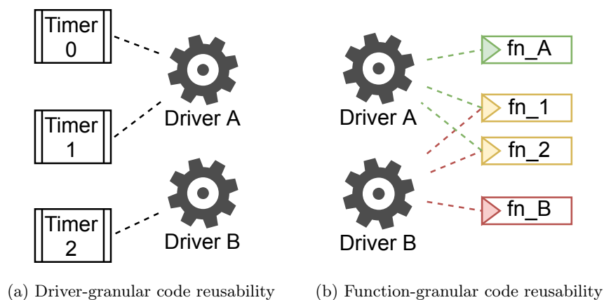
Figure 5.2: hAPI driver design concepts for code reusability
